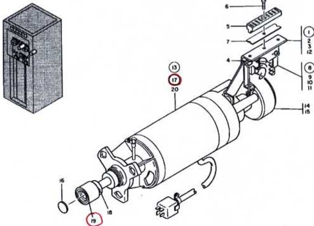
FIGURE 7. CAPSTAN MOTOR AND SENSING SWITCH ASSEMBLY. SEE LIST 7.
